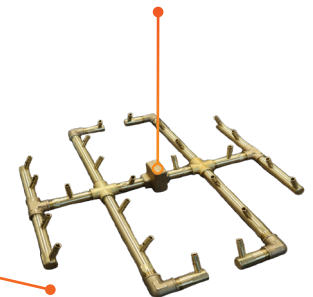
CROSSFIRE® Brass Burner (CFB180)
