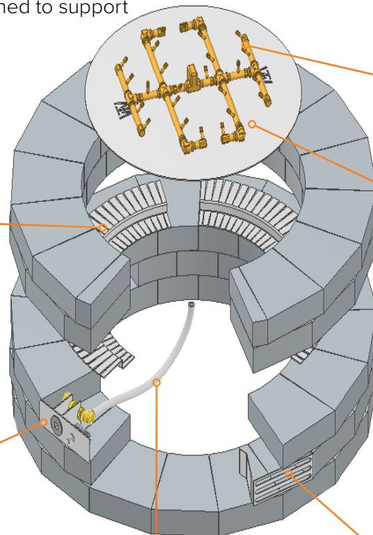
CROSSFIRE® Brass Burner (CFB180)
