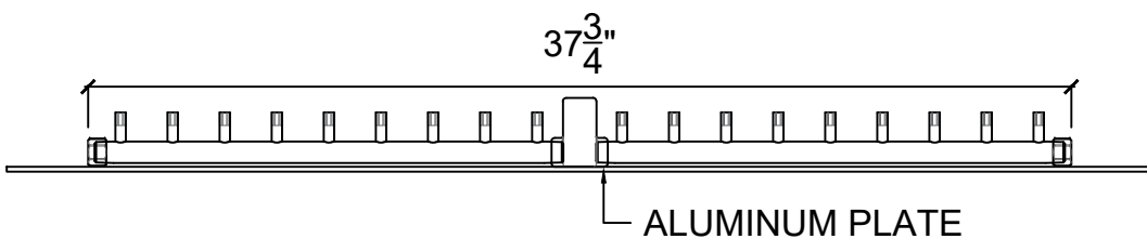
ELEVATION VIEW
