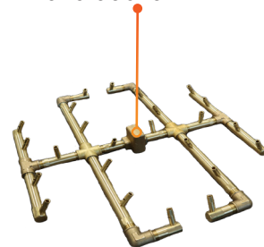
CROSSFIRE® Brass Burner (CFB240)
