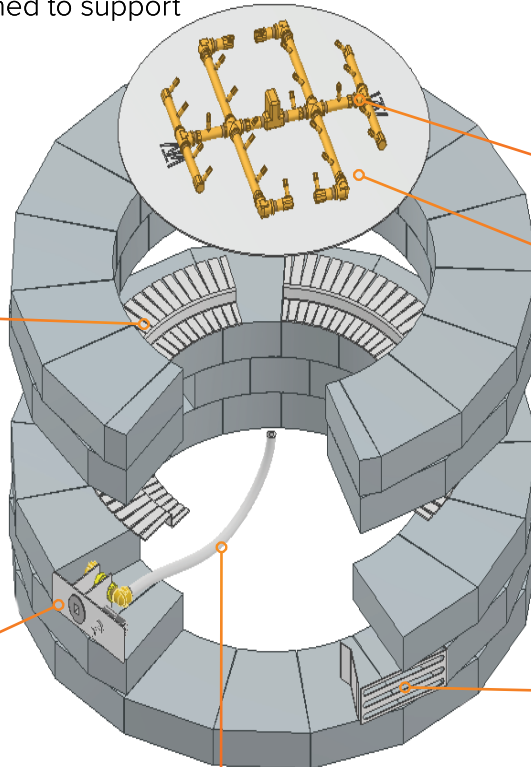
CROSSFIRE® Brass Burner (CFB240)
